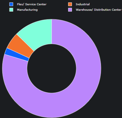
Sector Exposure
